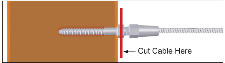
Figure P. Pull the cable tight to the lag stud end and cut it.
