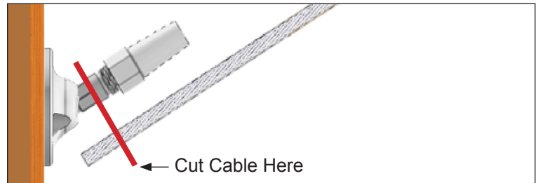
Figure Y Pull the cable tight to the tensioner, mark and cut the cable at the hex flats on the threaded stud.
