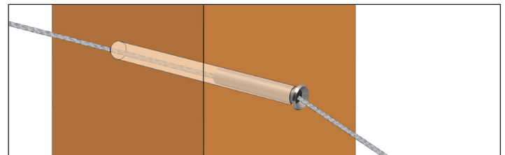
Figure AF. Cable Sleeve Diagram - Accommodating a stairway coming off a straight run.
