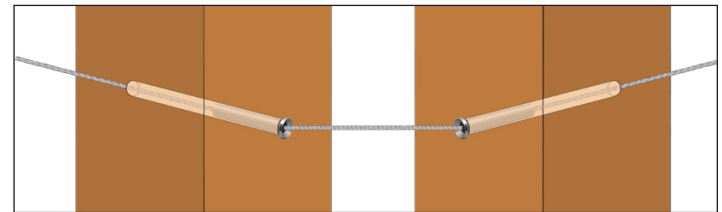
Figure AE. Cable Sleeve Diagram - Accommodating angles up to 90 degrees. Doubling up on corner posts is required.
