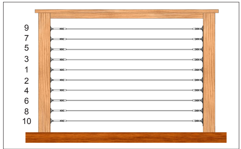
Figure Q. Tensioning Diagram - Begin with the center run of cable and alternate working above and below until cables are tight.
