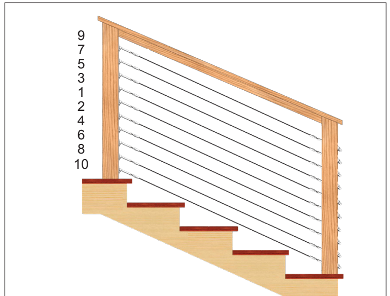
Figure AA. Tensioning Diagram - Begin with the center run of cable and alternate working above and below until cables are tight.
