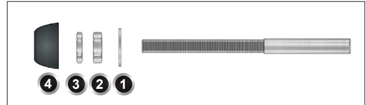
Figure AD. HandiSwage™ Cover Nut Set assembly diagram - 1) Stainless Steel Washer 2) Stainless Steel Nut 3) Stainless Steel Lock Nut & 4) HandiSwage™ Cover. RailEasy™ Stud Assembly not included.
