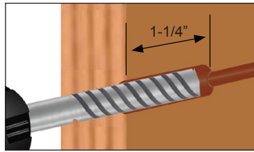
Figure L. (Left) Re-drill the back end of the post with a 3/8" bit approximately 1-1/4" deep to accept the flush fitting.
